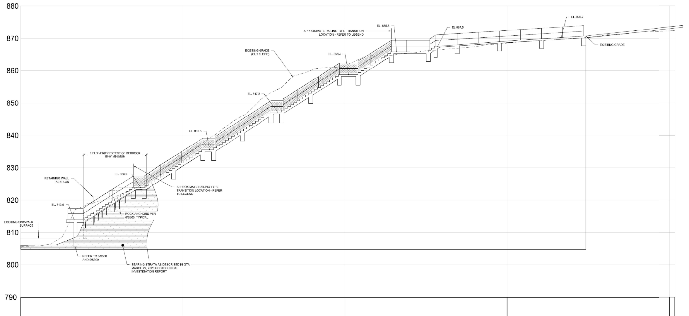
PROFILE FOR STAIRS PROFILE HORIZONTAL SCALE: 1" = 5' VERTICAL SCALE: 1" = 5'
