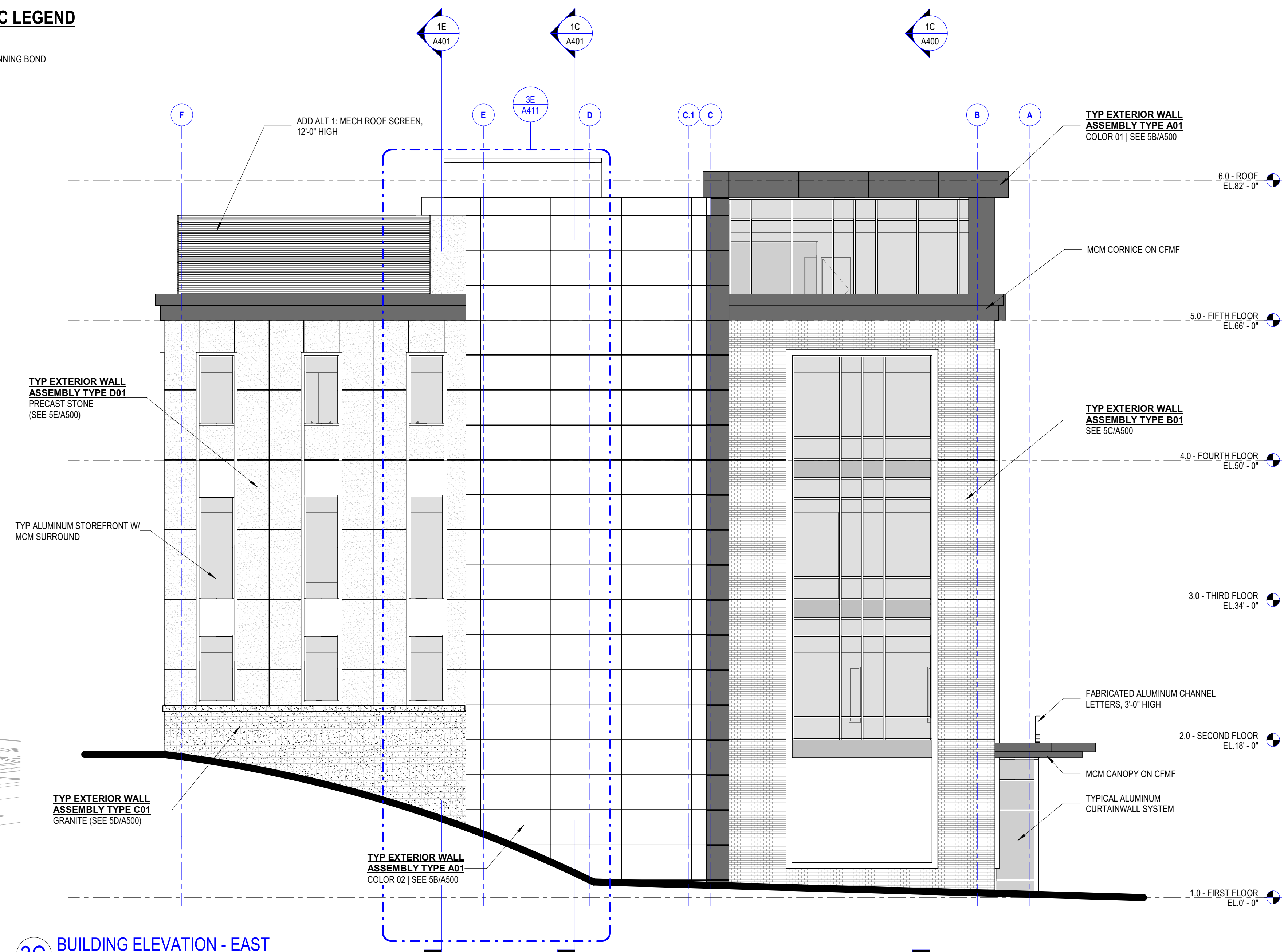
3C BUILDING ELEVATION - EAST 1/8" = 1'-0"
