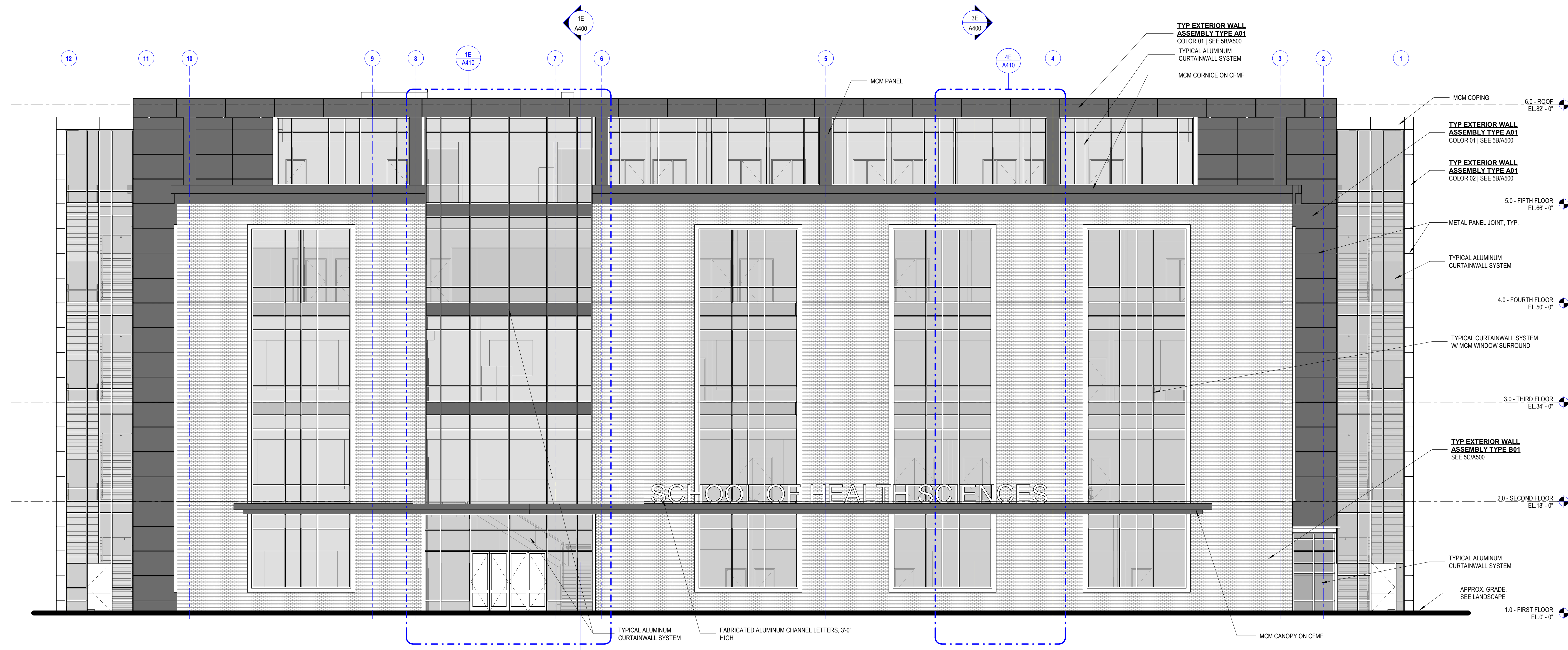
1E BUILDING ELEVATION - NORTH 1/8" = 1'-0"
