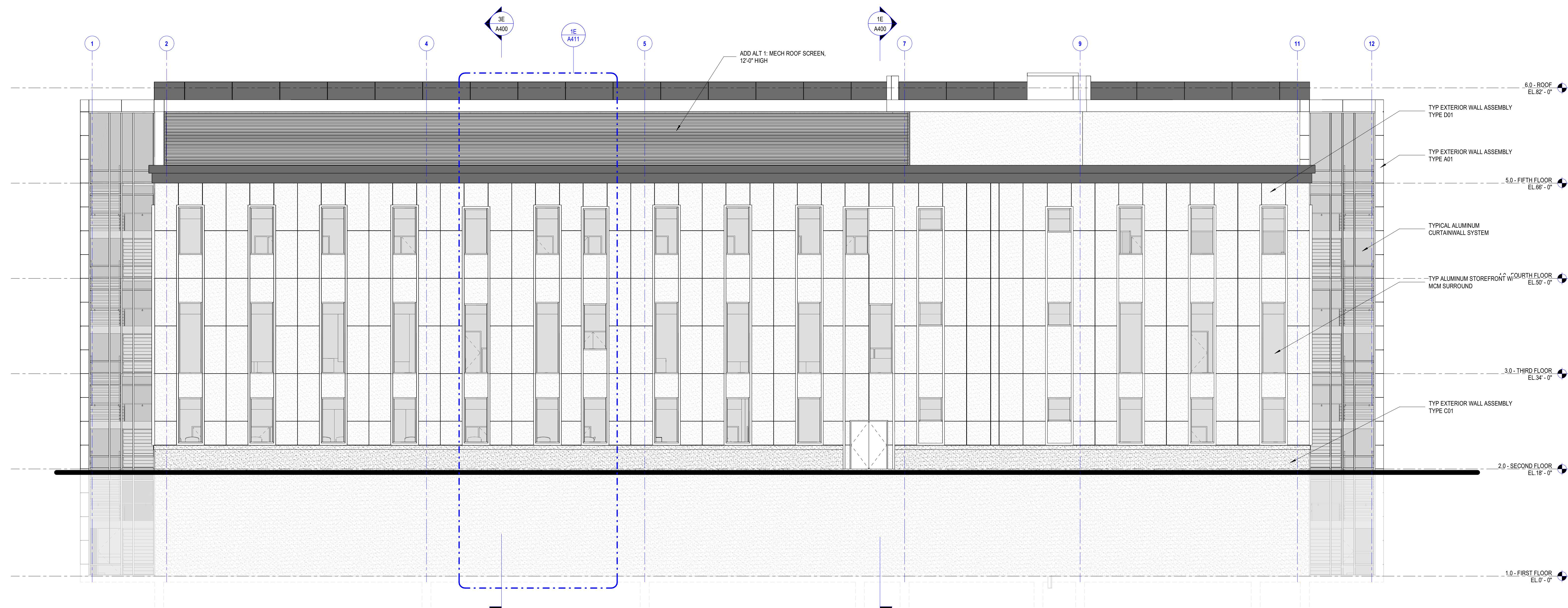
1E BUILDING ELEVATION - SOUTH 1/8" = 1'-0"
