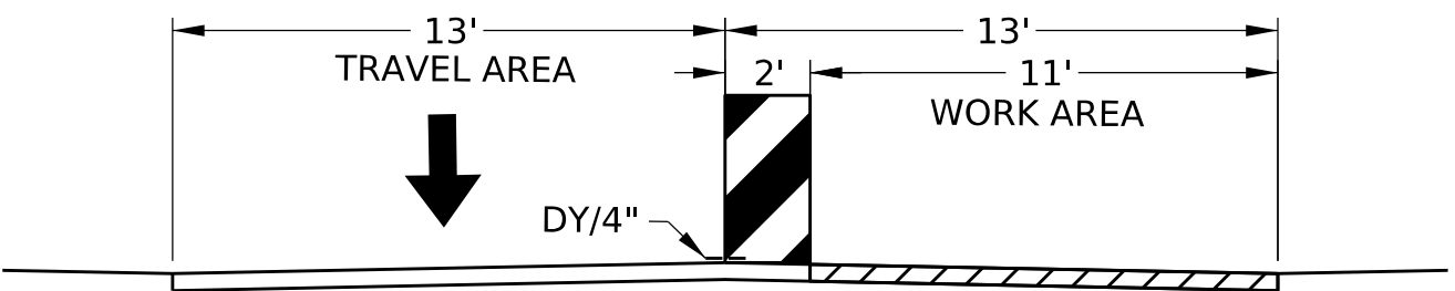
TYPICAL SECTION NOT TO SCALE
