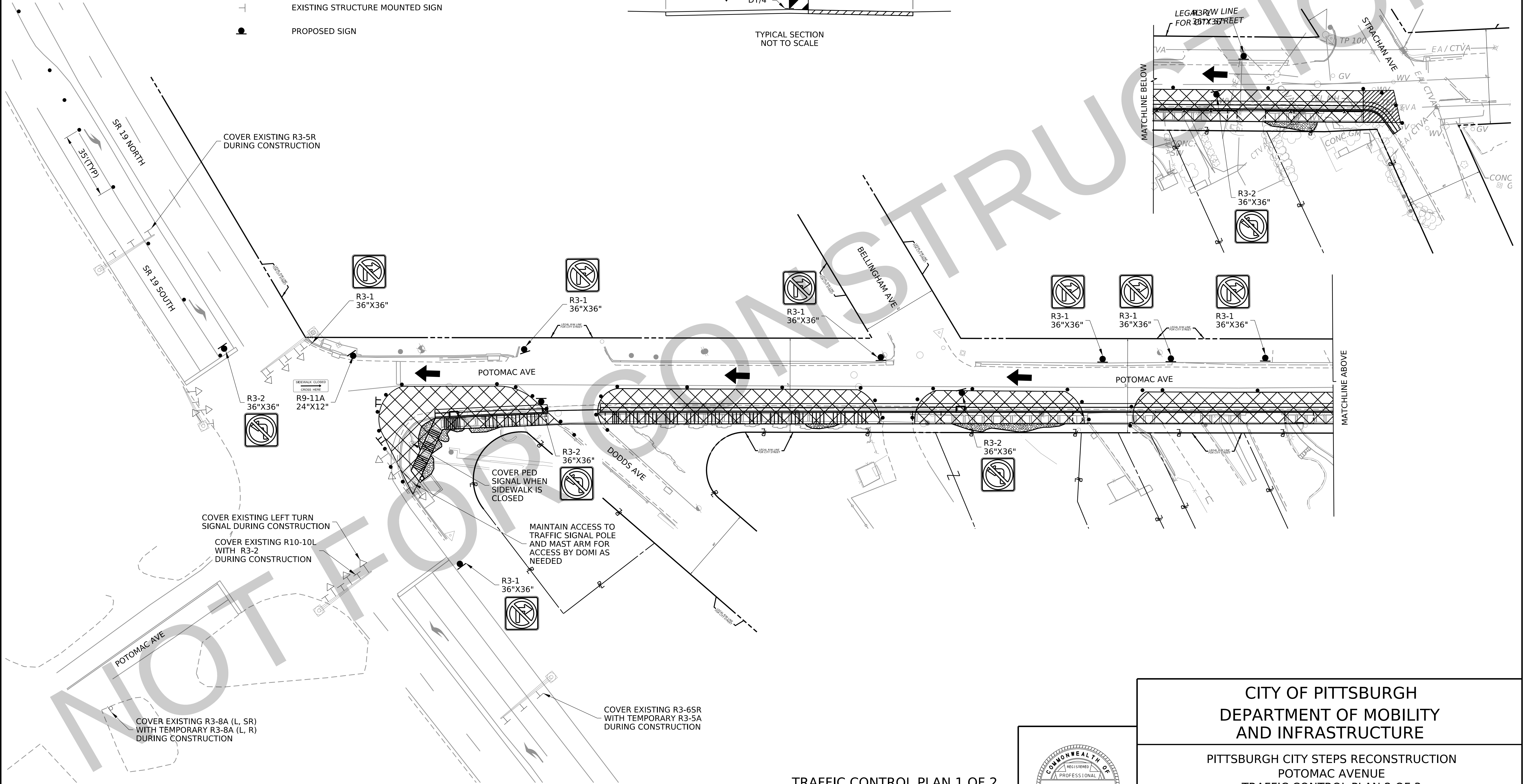
TRAFFIC CONTROL PLAN 1 OF 2
