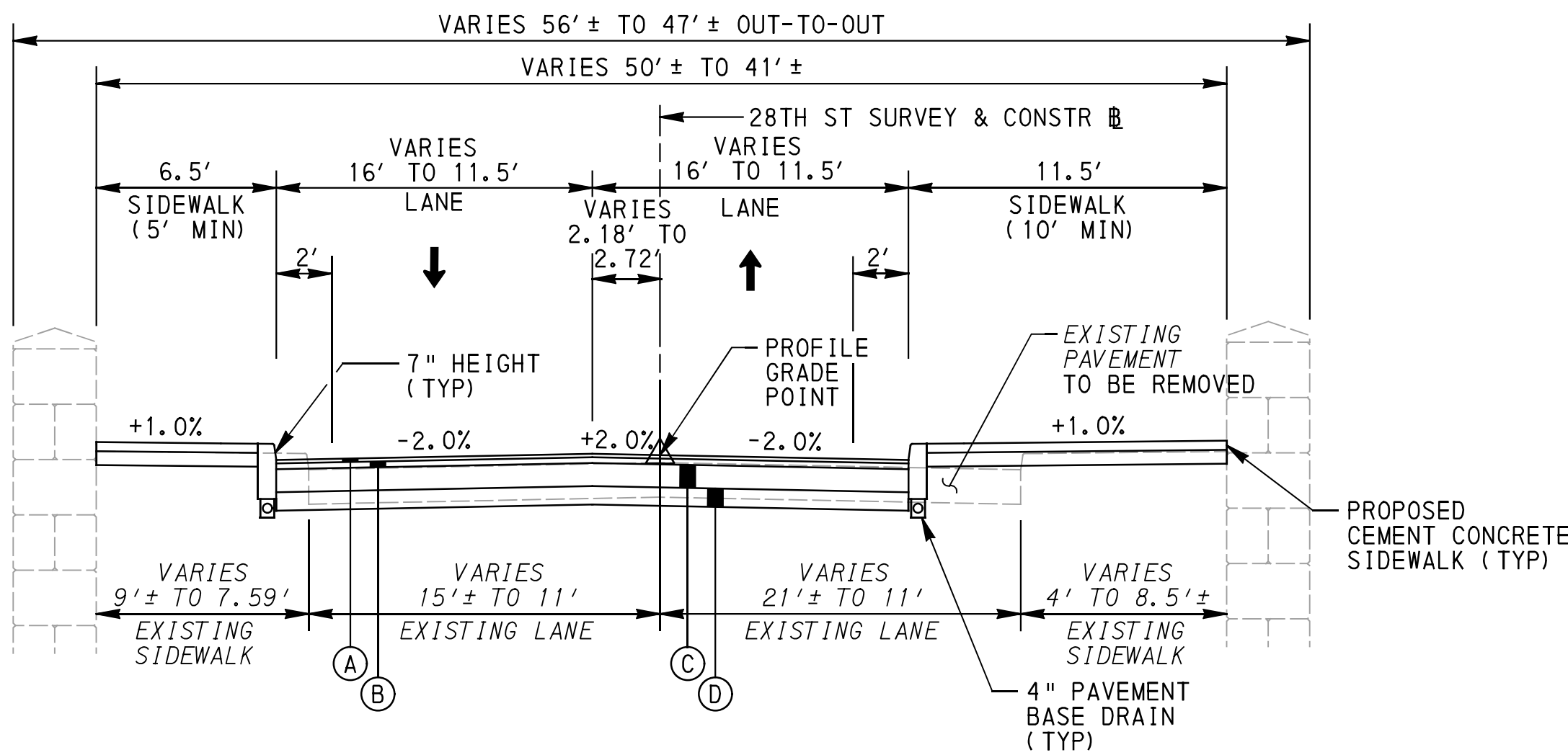
APPROACH ROADWAY TYPICAL SECTION - 28TH STREET
