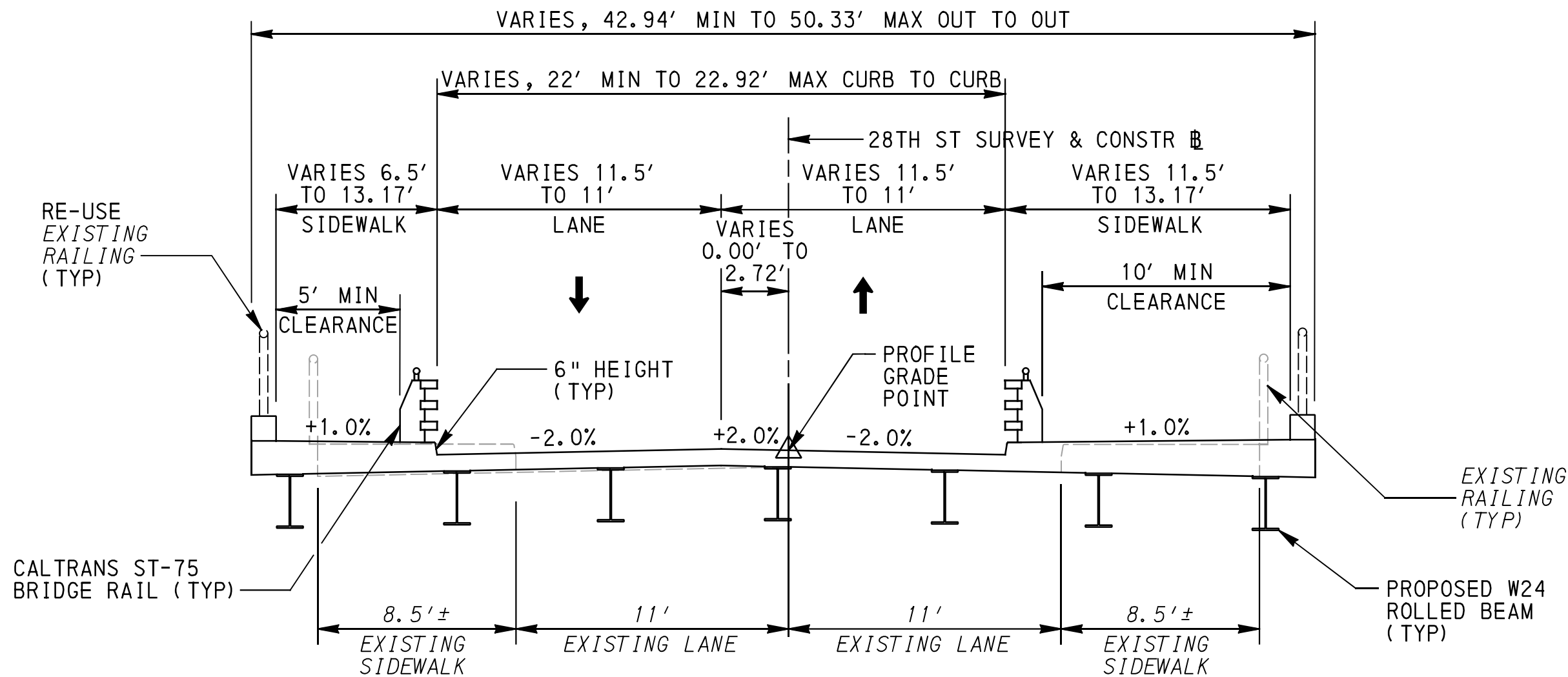
APPROACH BRIDGE TYPICAL SECTION - 28TH STREET
