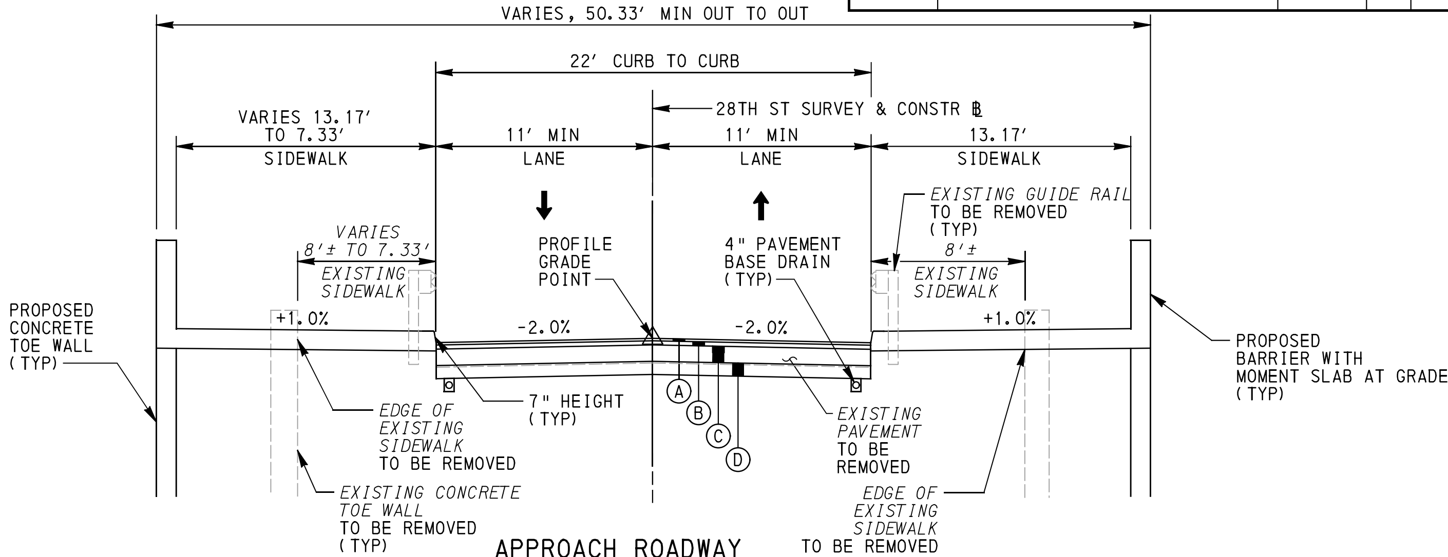
APPROACH ROADWAY TYPICAL SECTION - 28TH STREET
