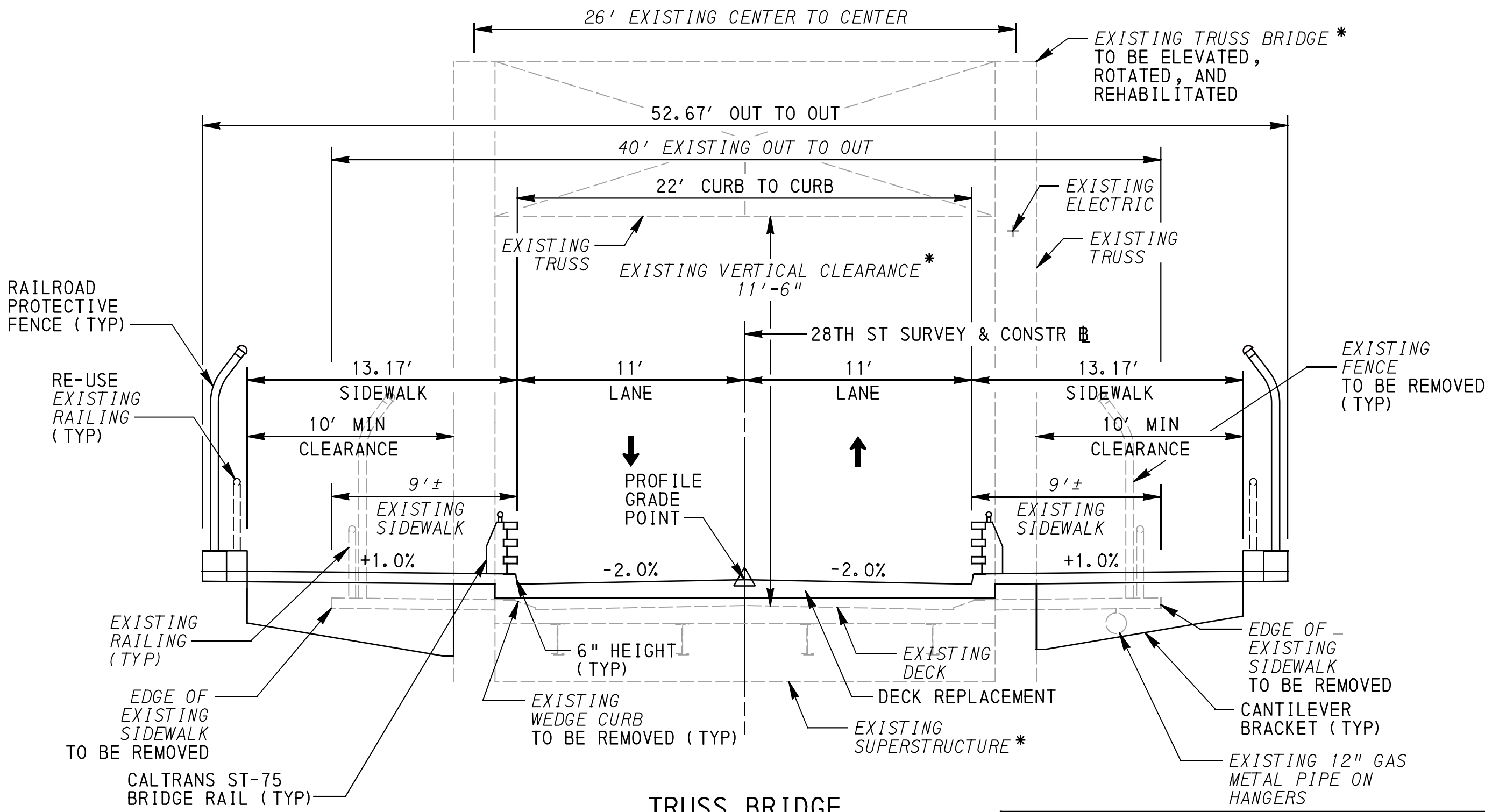
TRUSS BRIDGE TYPICAL SECTION - 28TH STREET
